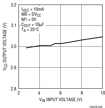
V CC Output Voltage vs Input Voltage (3V Mode)
