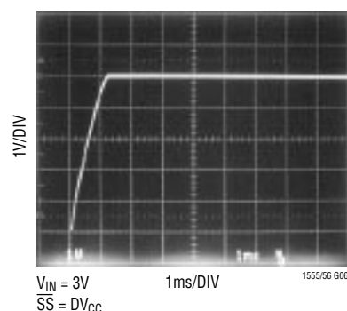
V CC Output Voltage Turn-On Time, SS Disabled
